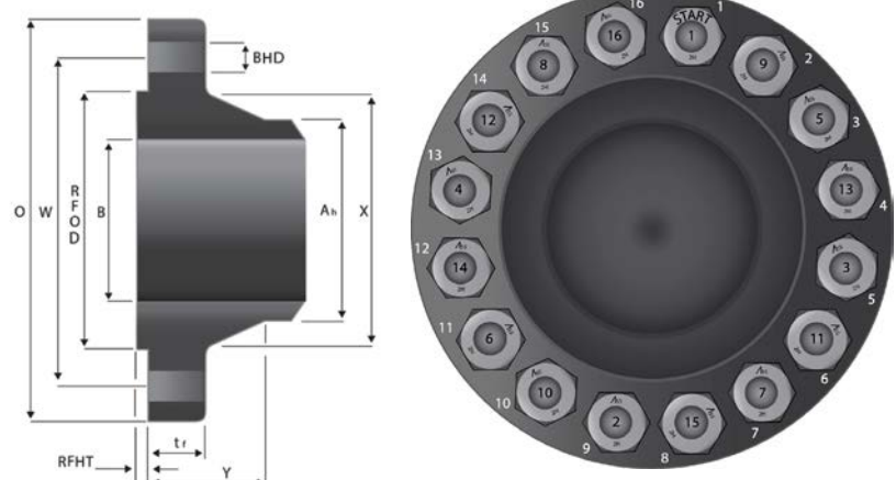
ASME B16.5 Raised Face Weld Neck Flange
